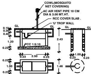
PLAN AND CROSS SECTION OF ST&SP.
