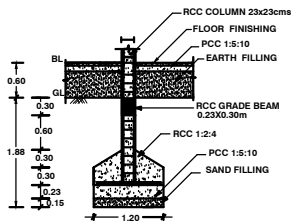
FOUNDATION DETAILS
