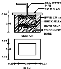
RAIN WATER COLLECTION TANK
