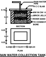
RAIN WATER COLLECTION TANK
