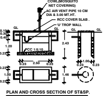
PLAN AND CROSS SECTION OF ST&P.
