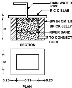
WATER COLLECTION TANK
