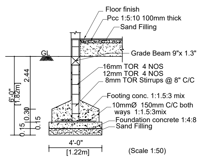
FOUNDATION DETAILS
