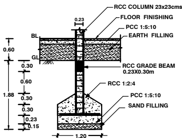
FOUNDATION DETAILS
