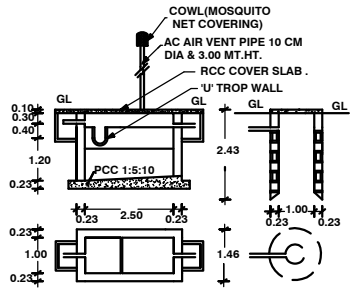
PLAN AND CROSS SECTION OF ST&P.
