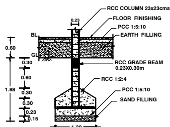
FOUNDATION DETAILS
