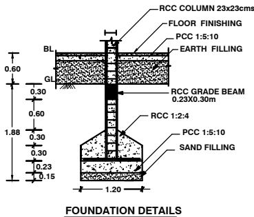
FOUNDATION DETAILS
