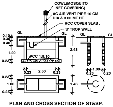
PLAN AND CROSS SECTION OF ST&SP.
