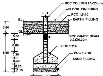
FOUNDATION DETAILS
