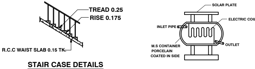
STAIR CASE DETAILS
