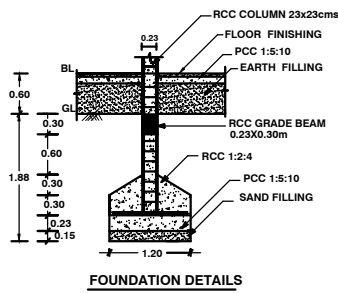
FOUNDATION DETAILS
