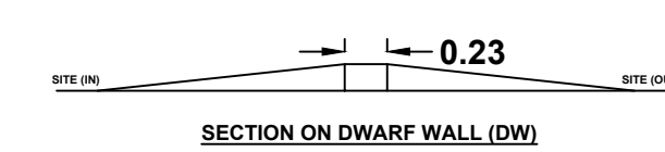
SECTION ON DWARF WALL (DW)
