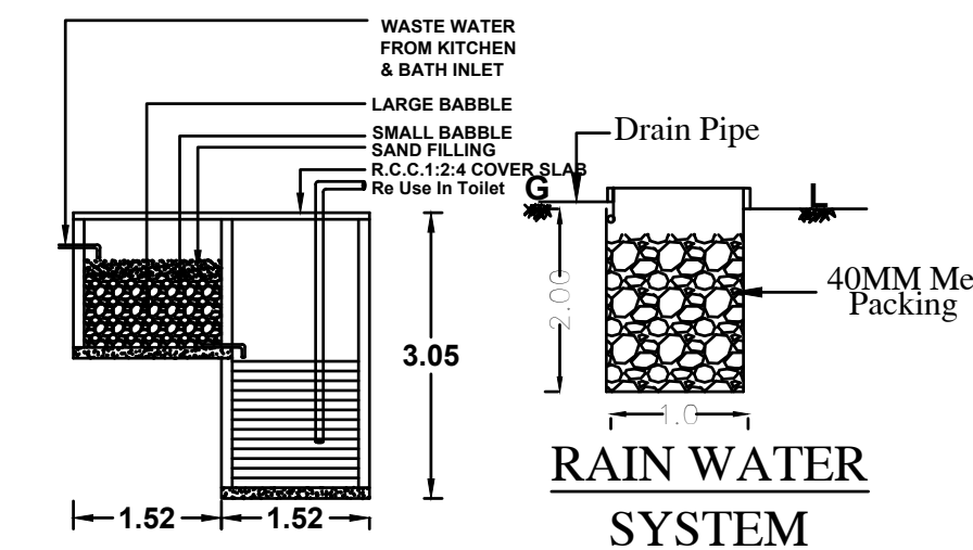
RECYCLING OF WASTE WATER FROM KITCHEN & BATHROOM
