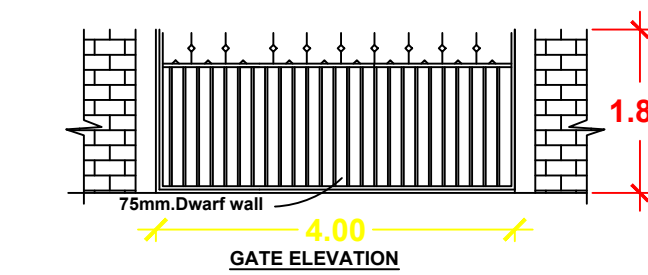
GATE ELEVATION
