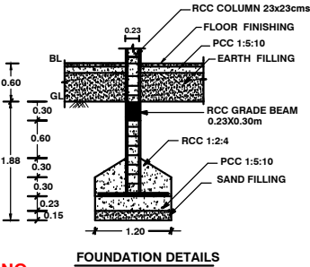
FOUNDATION DETAILS
