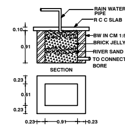
RAIN WATER COLLECTION TANK
