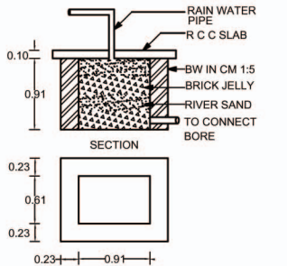
RAIN WATER COLLECTION TANK
