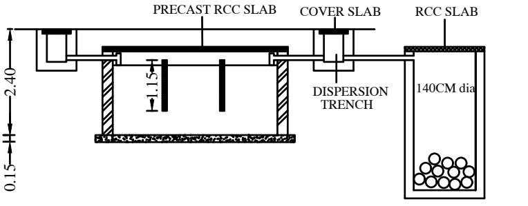
SECTION
