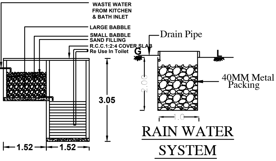
RECYCLING OF WASTE WATER FROM KITCHEN & BATHROOM
