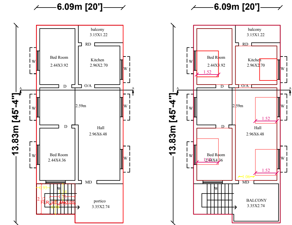
EXG.GROUND FLOOR
