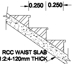
STAIR CASE STEPS SCALE 1:25
