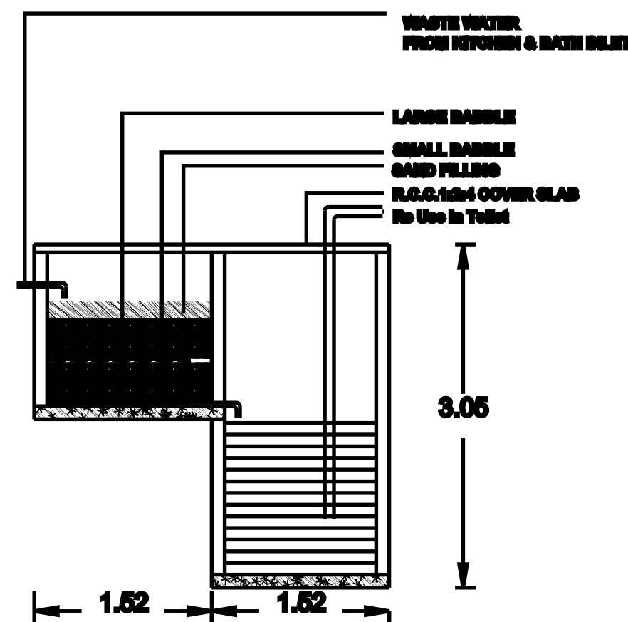
RECYCLING OF WASTE WATER FROM KITCHEN & BATH ROOM
