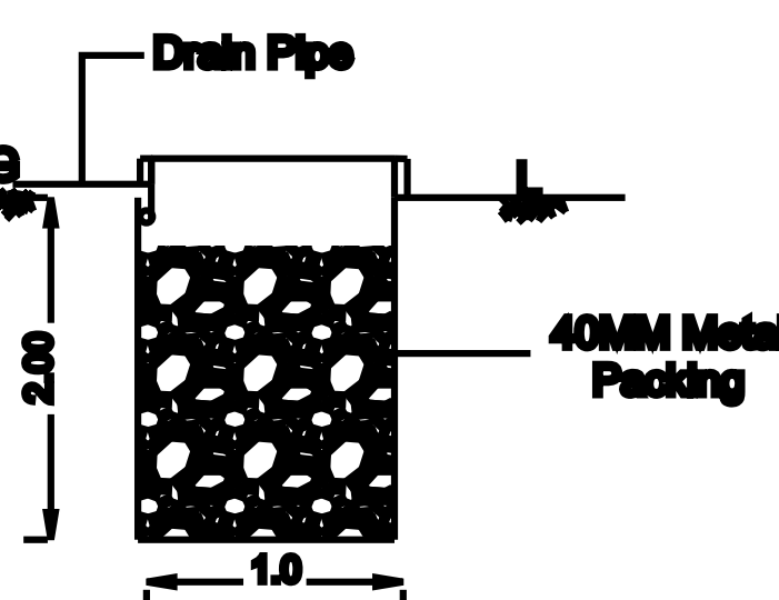
RAIN WATER SYSTEM
