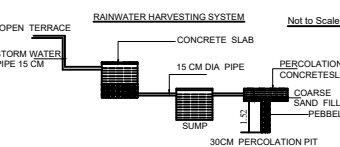
RAINWATER PERCOLATION PIT
