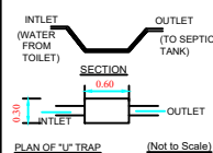
PLAN OF "U" TRAP (Not to Scale)
