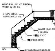
STAIRCASE DETAILS
