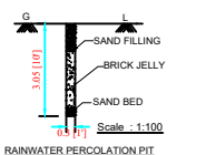
RAINWATER PERCOLATION PIT
