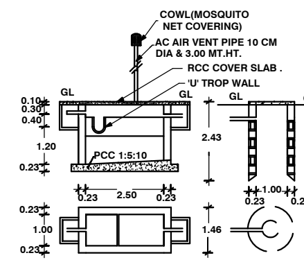
PLAN AND CROSS SECTION OF ST&SP.
