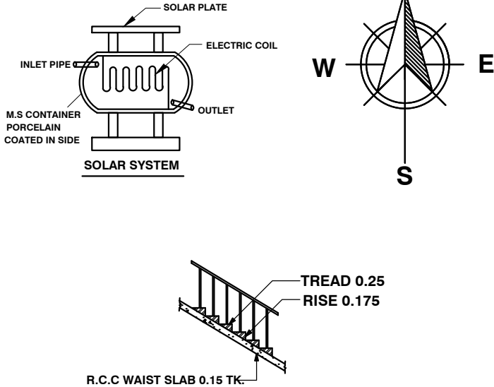
STAIR CASE DETAILS
