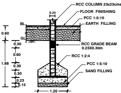
FOUNDATION DETAILS
