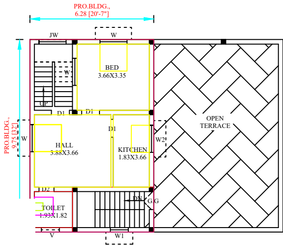
PRO.ADDL.FIRST FLOOR PLAN
