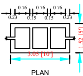
SEPTIC TANK DETAILS SCALE-1:100
