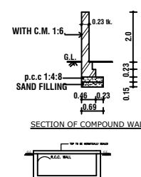
SECTION OF COMPOUND WALL
