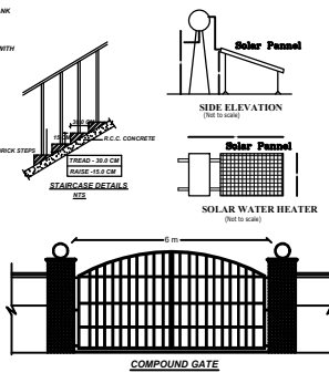
COMPOUND GATE
