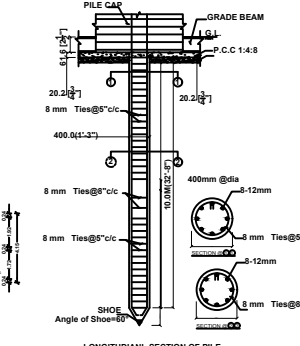
LONGITUDINAL SECTION OF PILE
