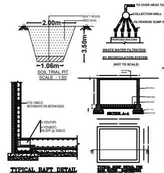
TYPICAL RAFT DETAIL
