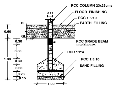
FOUNDATION DETAILS
