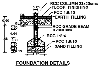
FOUNDATION DETAILS
