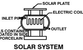
SOLAR SYSTEM
