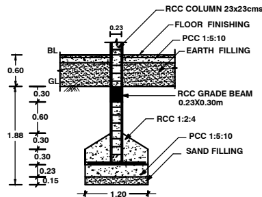
FOUNDATION DETAILS
