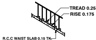
STAIR CASE DETAILS
