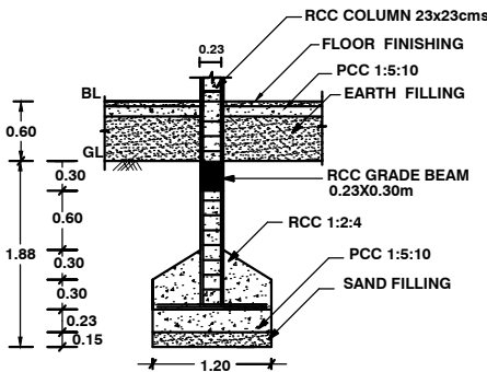
FOUNDATION DETAILS
