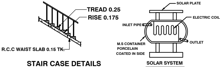
STAIR CASE DETAILS
