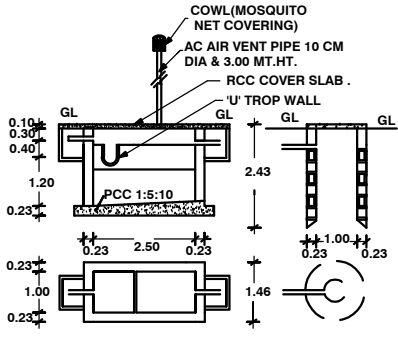
PLAN AND CROSS SECTION OF ST&SP.
