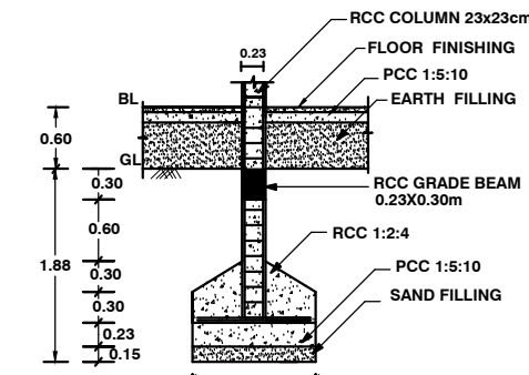
FOUNDATION DETAILS
