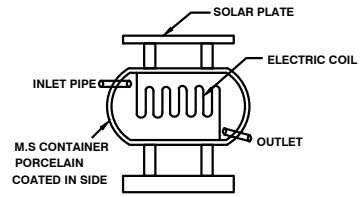
SOLAR SYSTEM
