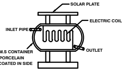
SOLAR SYSTEM
