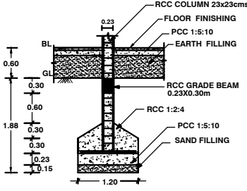
FOUNDATION DETAILS
