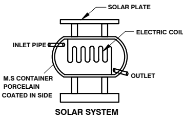
SOLAR SYSTEM
