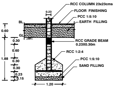
FOUNDATION DETAILS
