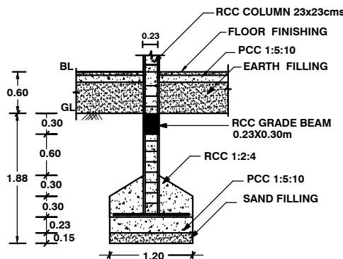
FOUNDATION DETAILS
