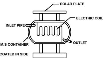
SOLAR SYSTEM
