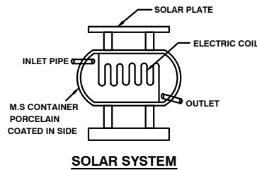
SOLAR SYSTEM
