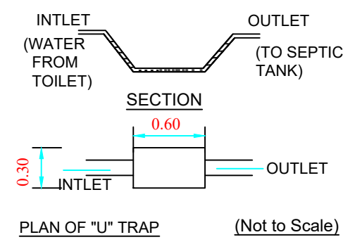
PLAN OF "U" TRAP
