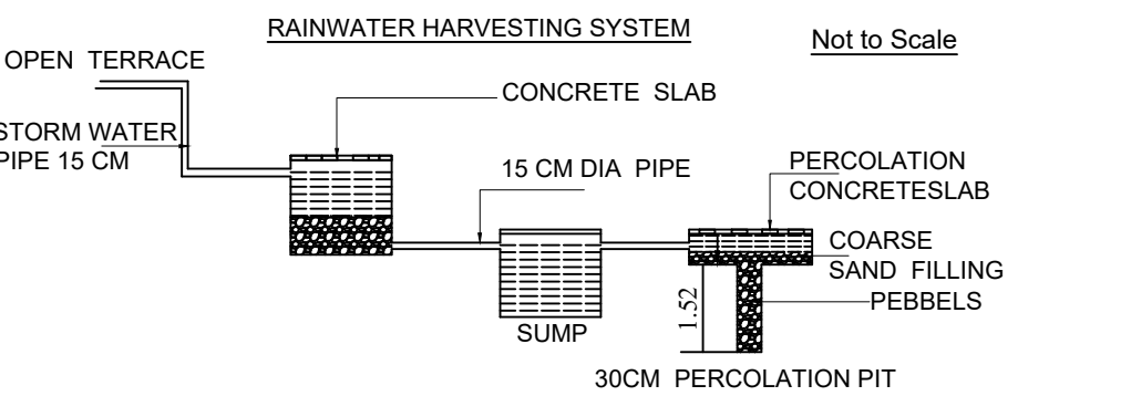
RAINWATER PERCOLATION PIT
