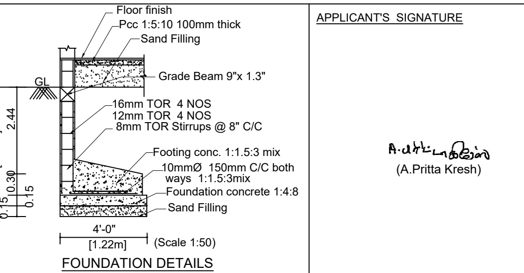
FOUNDATION DETAILS
