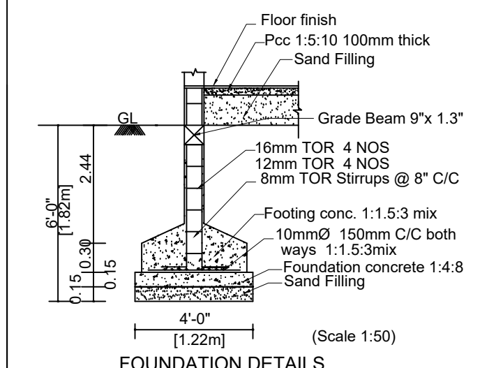
FOUNDATION DETAILS
