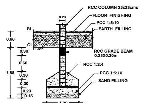
FOUNDATION DETAILS
