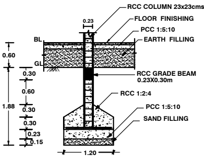
FOUNDATION DETAILS
