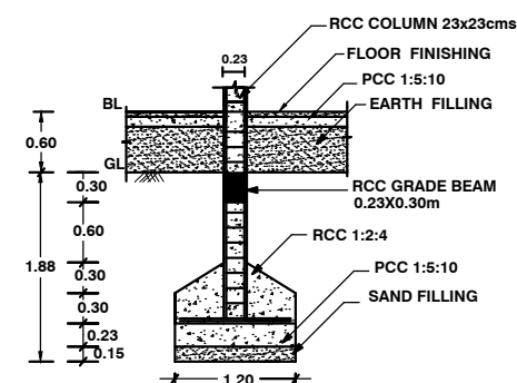
FOUNDATION DETAILS
