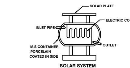
SOLAR SYSTEM
