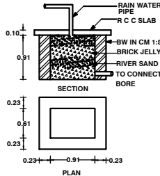
RAIN WATER COLLECTION TANK
