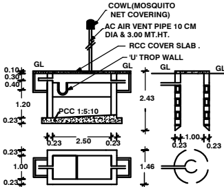
PLAN AND CROSS SECTION OF ST&SP.
