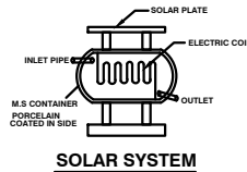
SOLAR SYSTEM
