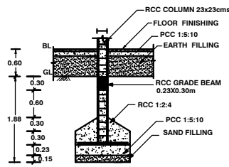
FOUNDATION DETAILS
