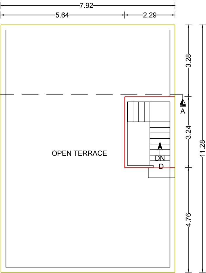
HEAD ROOM PLAN
