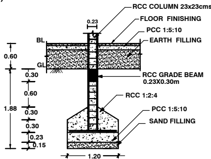
FOUNDATION DETAILS
