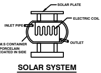
SOLAR SYSTEM
