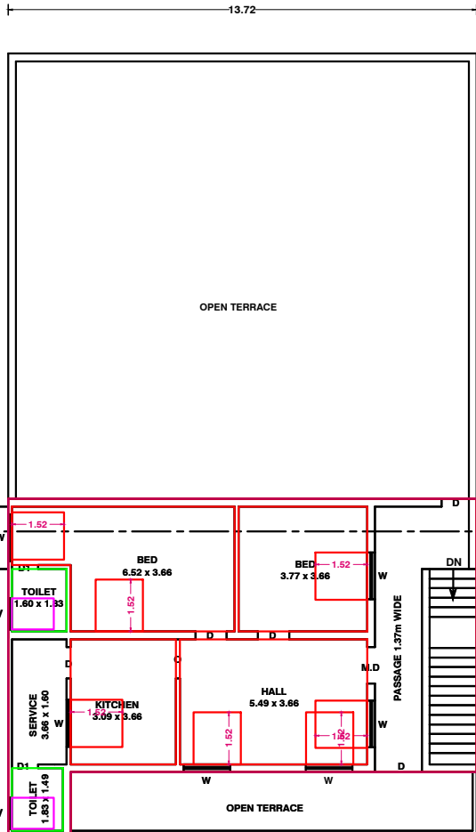
PRO. SECOND FLOOR PLAN
