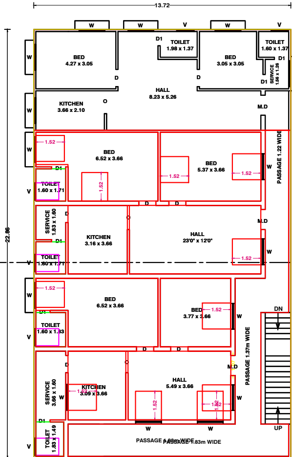
EXIST. & PRO. FIRST FLOOR PLAN
