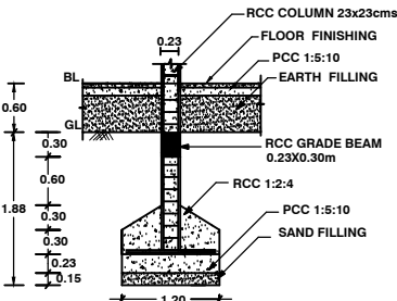
FOUNDATION DETAILS
