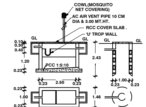
PLAN AND CROSS SECTION OF ST&SP.
