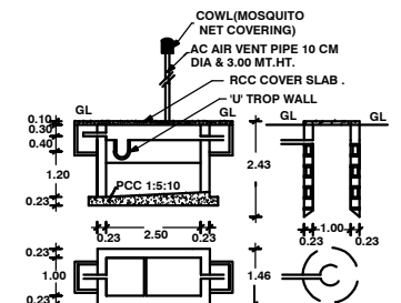
PLAN AND CROSS SECTION OF ST&SP.
