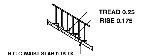
STAIR CASE DETAILS
