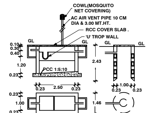
PLAN AND CROSS SECTION OF ST&SP.
