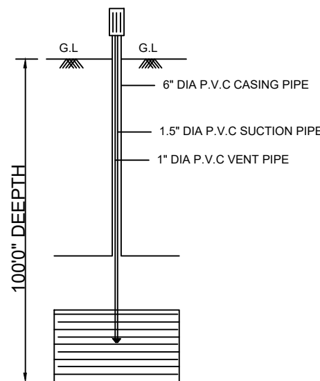
BORE WELL
