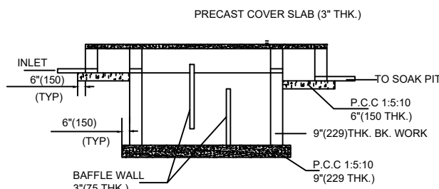
SECTION - BB
