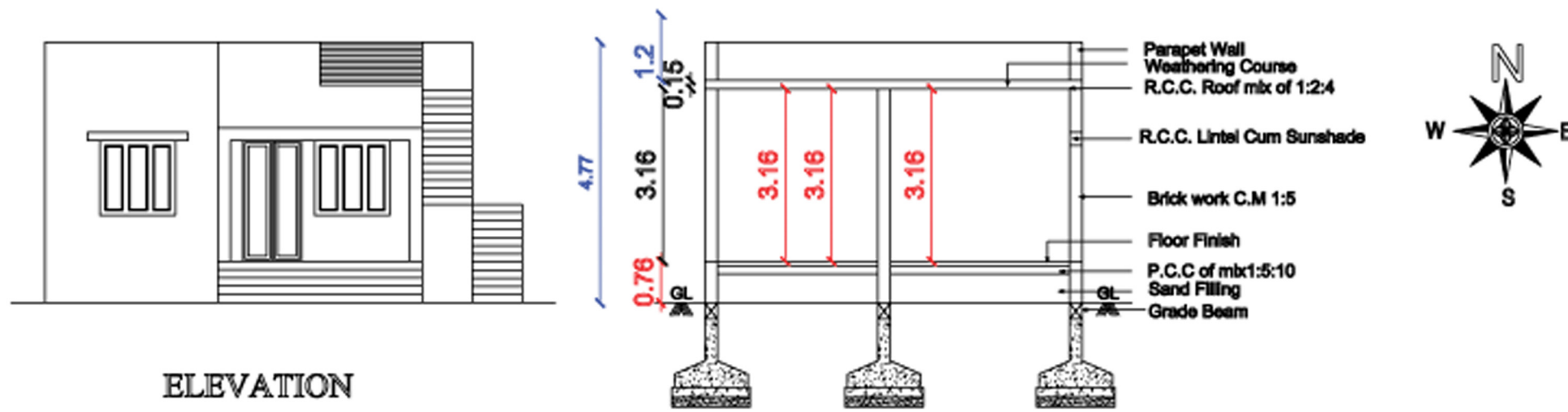
CROSS SECTION AB
