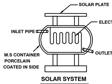
SOLAR SYSTEM
