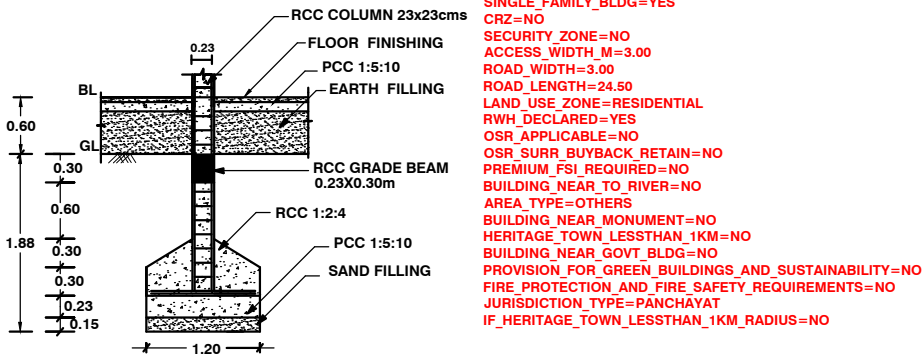
FOUNDATION DETAILS
